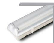
Model : PEL 240 M/SL Lamp Type : 2 x 36/40W FTL Accumulator : SLA Battery Backup : 1 Hrs. Standard Pkg.: 2 pcs. Box size in mm : 310x170x1290
