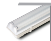
Model : PEL 220 M/SL Lamp Type : 2 x 18/20W FTL Accumulator : SLA Battery Backup : 1 Hrs. Standard Pkg.: 2 pcs. Box size in mm : 275x200x740
