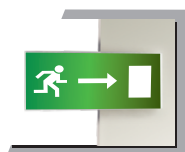
Model : PEL LED E/M (SC) Lamp Type : LED Accumulator : Ni-Cd Battery Backup : 3 Hrs. Standard Pkg.: 4 pcs. Box size in mm : 420x225x415
